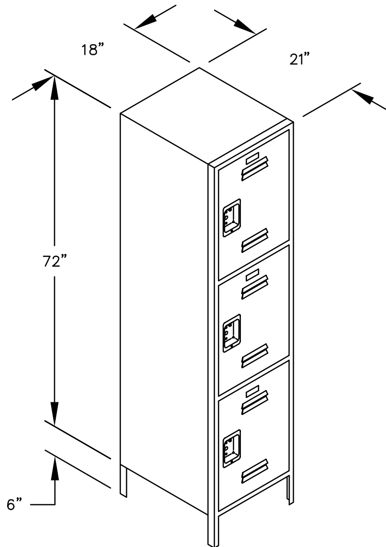
MODEL #18-53161 18" WIDE TRIPLE TIER STANDARD LOCKER – 1 WIDE
