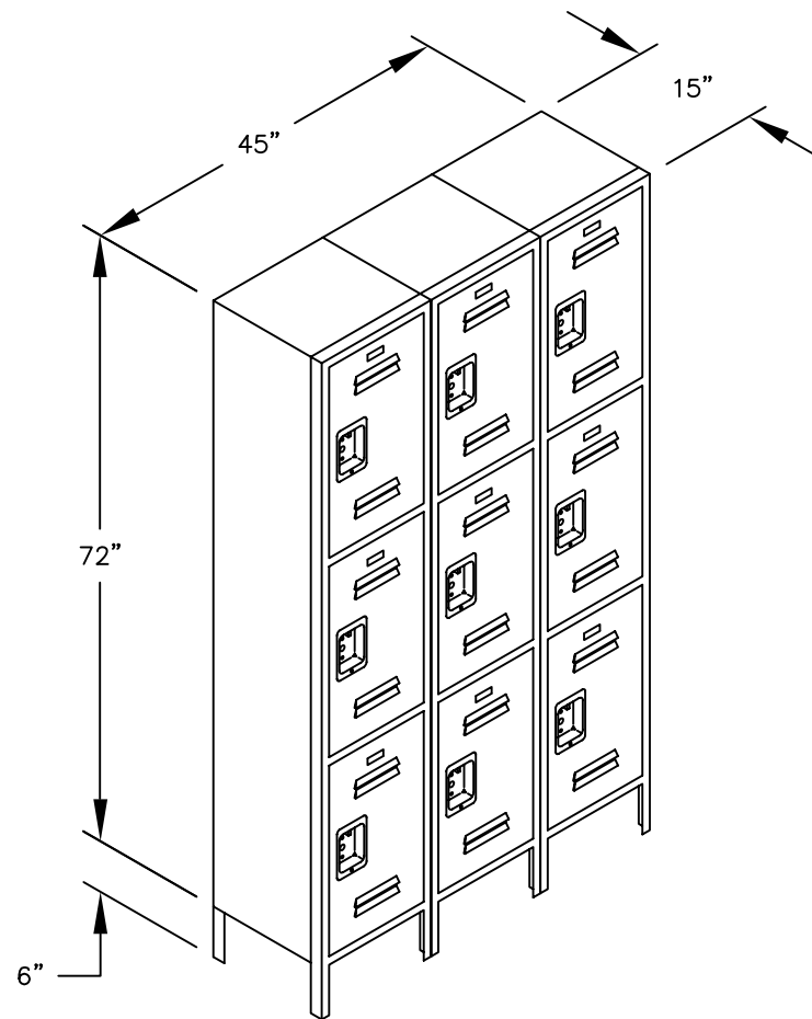
MODEL #53365 15" WIDE TRIPLE TIER STANDARD LOCKER – 3 WIDE
