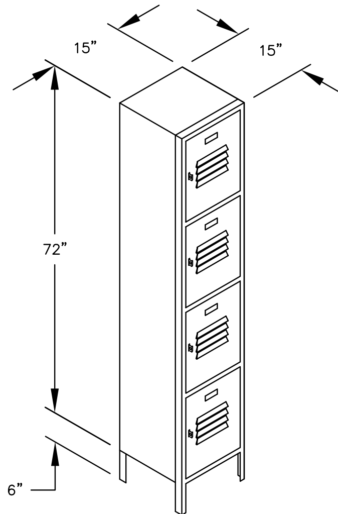
MODEL #54165 15" WIDE FOUR TIER STANDARD LOCKER – 1 WIDE
