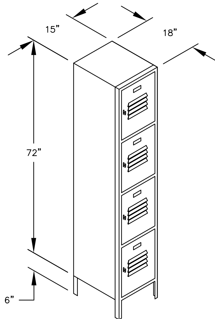
MODEL #54168 15" WIDE FOUR TIER STANDARD LOCKER – 1 WIDE
