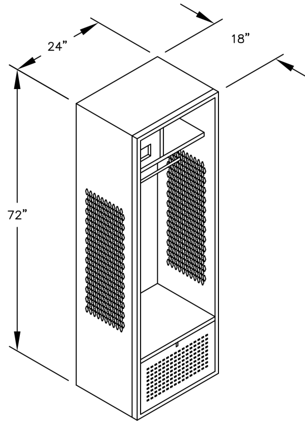
MODEL #70018 OPEN ACCESS STANDARD LOCKER
