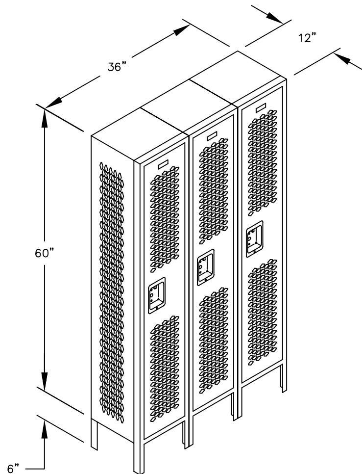
MODEL #71352 12" WIDE SINGLE TIER VENTED METAL LOCKER – 3 WIDE
