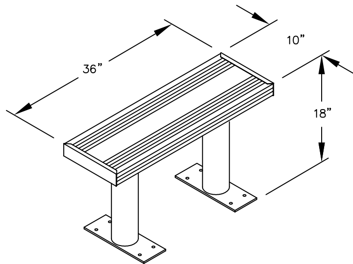
MODEL #77773 36" WIDE ALUMINUM LOCKER BENCH 36" W x 18" H x 10" D
