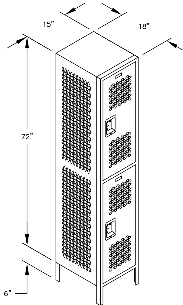
MODEL #82168 15" WIDE DOUBLE TIER VENTED METAL LOCKER – 1 WIDE
