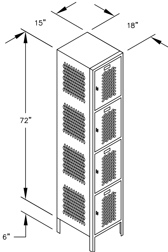
MODEL #84168 15" WIDE FOUR TIER VENTED METAL LOCKER – 1 WIDE
